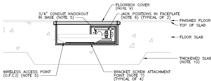
DETAIL 7C/T310 FLOOR BOX FOR WIRELESS ACCESS POINT SIDE VIEW (FACEPLATE) SCALE: 2"=1'-0"
