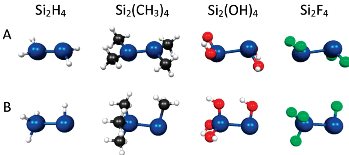
Figure 3. Locally optimized \text{Si}_2\text{L}_4 structures with L = \text{H}, \text{CH}_3, \text{OH}, \text{F} .
